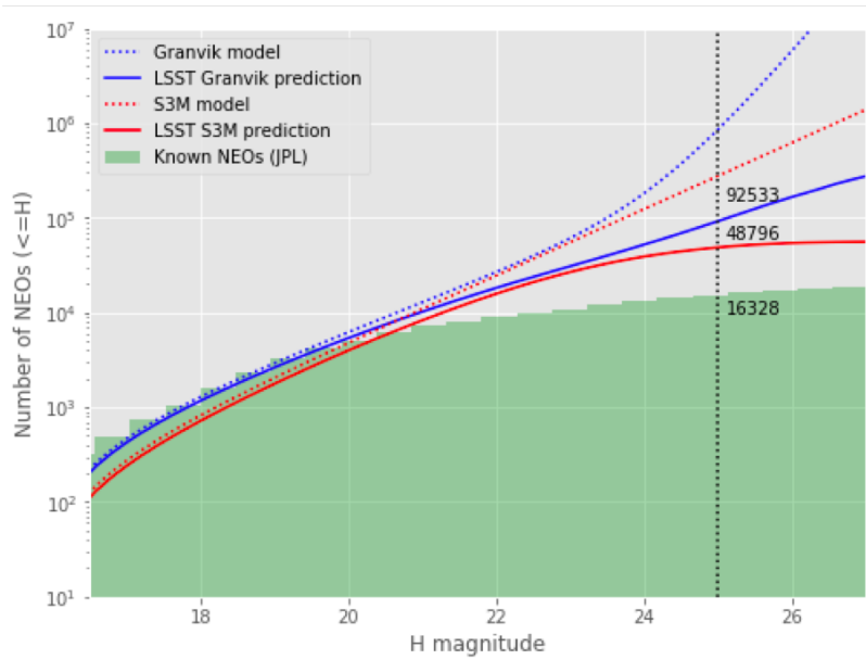
FIGURE 5: Number of NEOs discovered with the LSST for different population models (S3M, Grav et al., 2011) and Granvik et al. (2018). The prediction curves represent the cumulative number of discovered NEOs as a function of their absolute magnitude H , while the model curves show the number of expected objects in the population.
