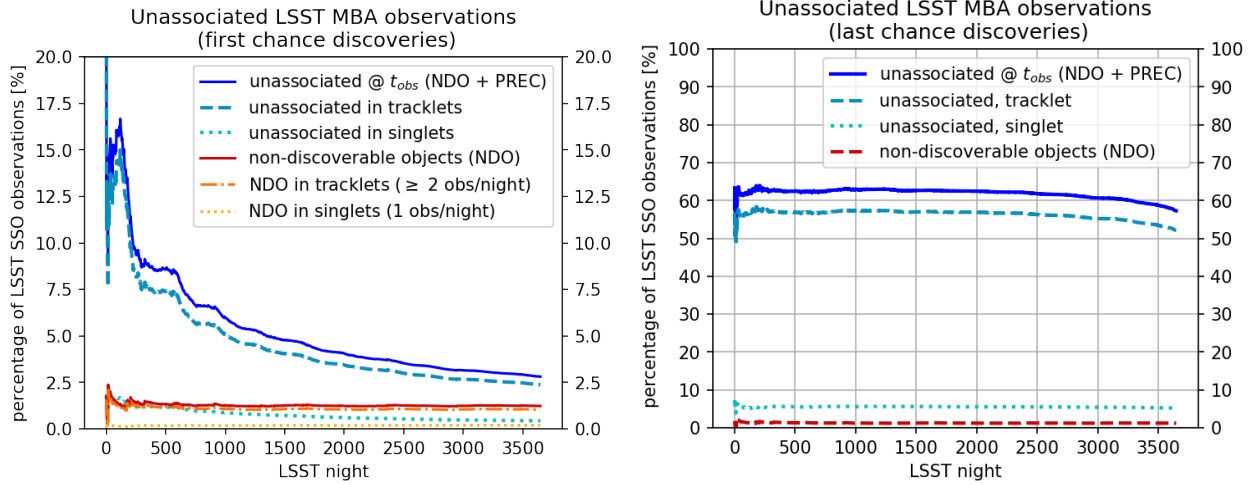
FIGURE 17: The fraction of unassociated and non-discoverable object observations with respect to all MBA observations is shown. In the graph on the left we assume all asteroids have been discovered at the first opportunity. In the graph on the right all asteroids have been discovered at the last opportunity.
