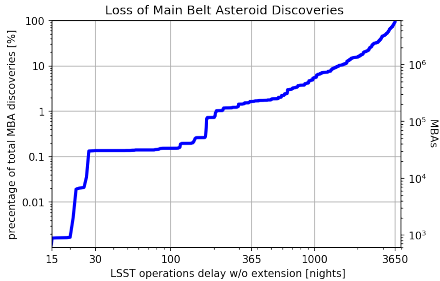
FIGURE 15: Losses in MBA discoveries due to delayed operations of the LSST (assuming no extension) for population model A.
