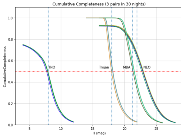
FIGURE 22: Cumulative completeness for various solar system populations with the Feature Based Scheduler 1.2 baseline. The two lines show results with visit pairs in the same filter vs. pairs in different filters (TNOs with C colors)
