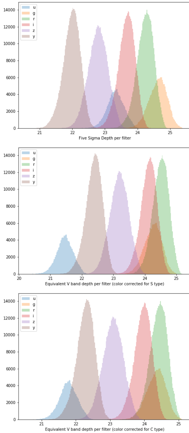
FIGURE 3: A comparison of LSST depths per filter for a flat SED (top), an SED corrected for S-type asteroids (center) and C-type asteroids (bottom), respectively. The number of LSST visits is shown on the y-axis. Values on the x-axis are given in magnitudes.
