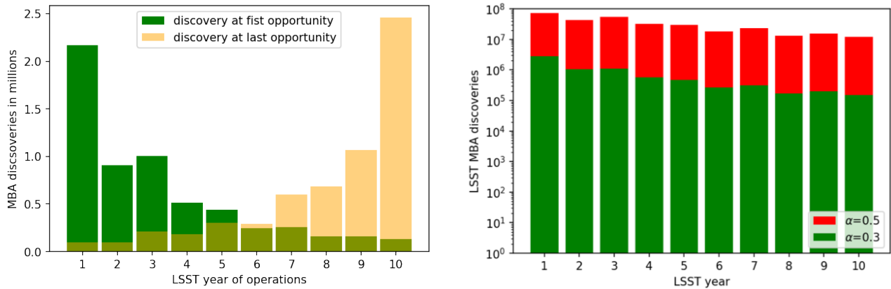
FIGURE 11: LSST Main Belt Asteroid (MBA) discoveries per year on a linear (left) and logarithmic scale (right) assuming 100% linking efficiency. The left panel compares yields for early and late discovery scenarios. The right panel shows discovery yields for population models A (green) and B (red) in an early discovery scenario.
