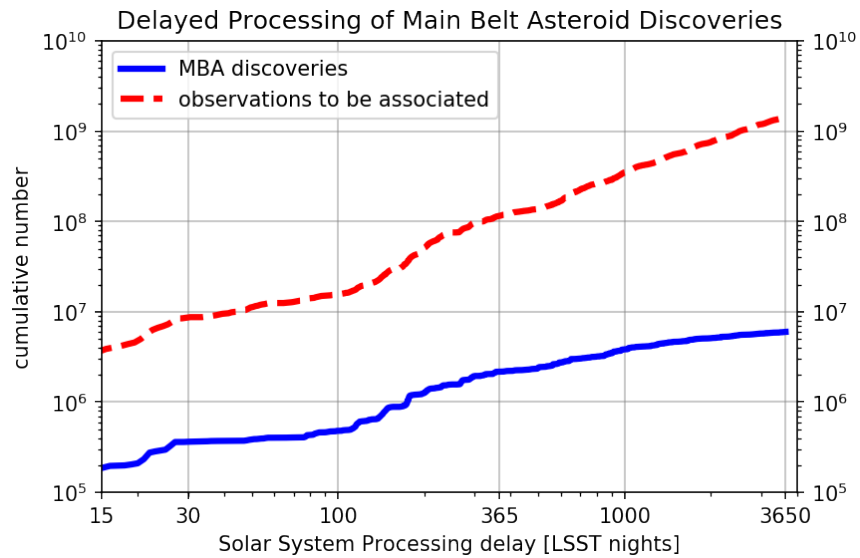
FIGURE 14: Cumulative number of MBAs (blue) and observations (red) that require reprocessing if SSP is delayed.
